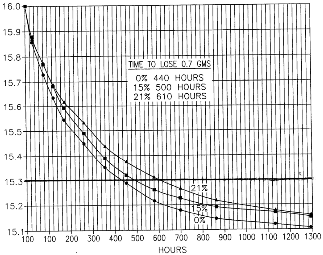
Figure 2: Reduced rate of loss of weight with increase concentration of nano-clay - MBN
