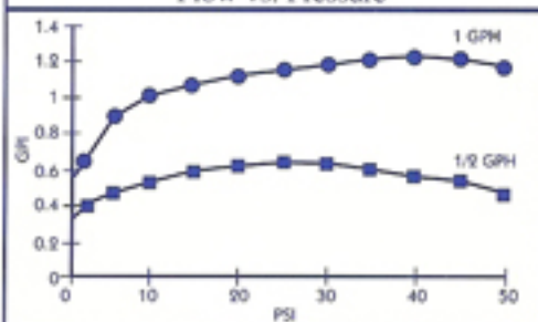
Flow vs. Pressure
